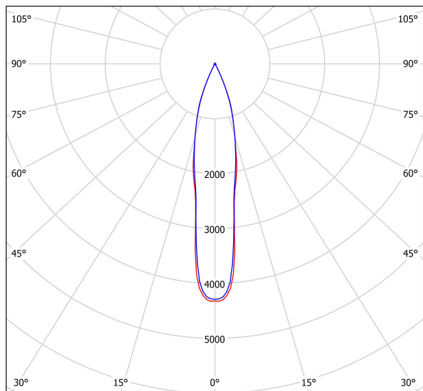
cd/klm \eta = 90\% — C0 - C180 — C90 - C270
