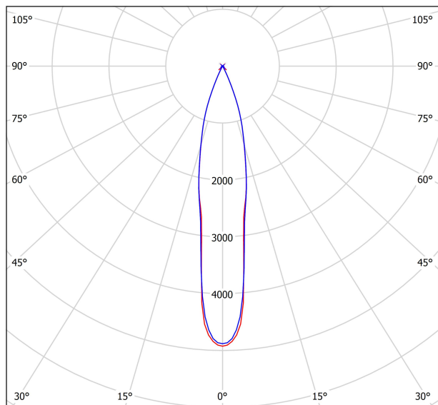
cd/klm — C0 - C180 — C90 - C270 η = 90%
